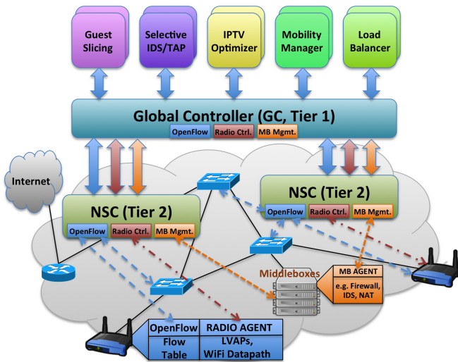
Figure 1: AeroFlux: NSCs are deployed close to the APs.
